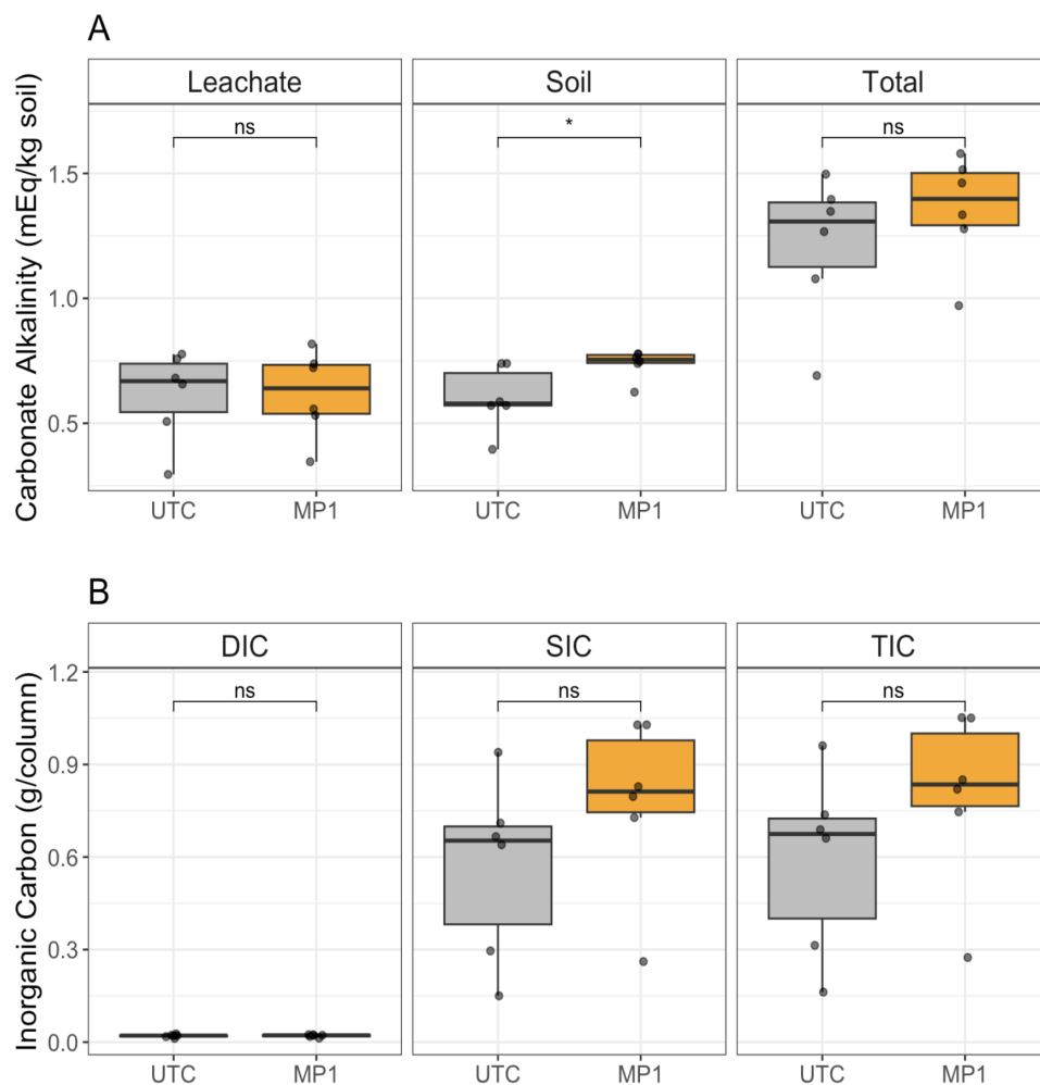
Figure 2: Carbonate alkalinity (A) and inorganic carbon (B) in MP1-treated and untreated control (UTC) columns. Student's t-test, * p < 0.05 , ns: not significant, N = 6 .
