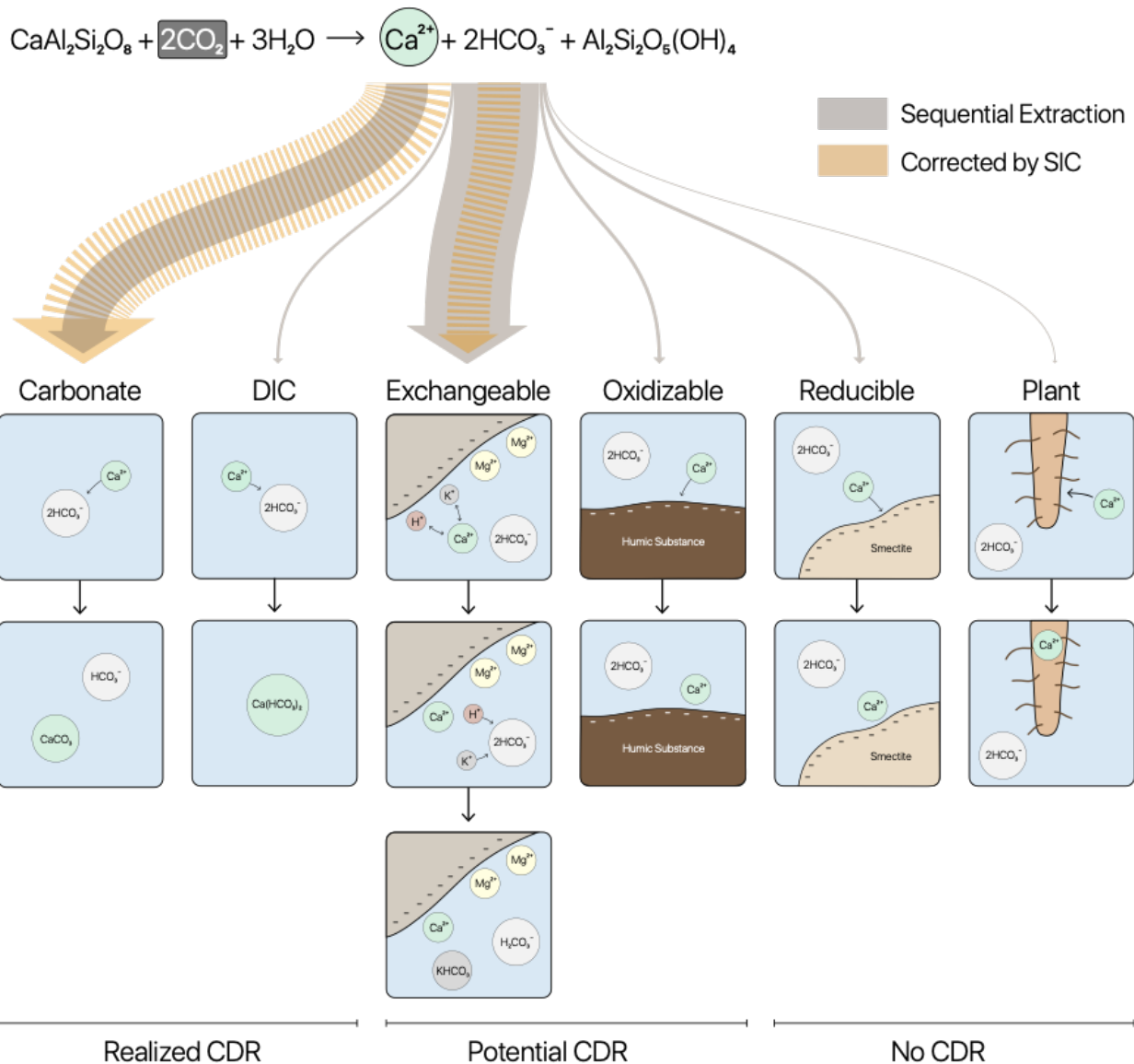
385 Figure 7: The mass balance approach reported here allows for tracking the fate of the observed increases in base cations from the acceleration of silicate weathering by B. subtilis MP1. For simplification, we assume the observed increase in Ca ions is derived from the dissolution of anorthite mineral, and that the resulting Ca ions end up in one of the six possible soil fractions: Carbonate, DIC, Exchangeable, Oxidizable, Reducible and Plant. The width of the gray arrows is proportional to the amount of new Ca ions that end 390 up in one of the six characterized soil fractions. The width of the yellow arrows is proportional to the amount of new Ca ions that end up in the exchangeable and carbonate pools, corrected by the soil inorganic carbon measurement. Only Ca ions that end up in the carbonate pool or are exported as dissolved inorganic carbon constitute “realized CDR”. The exchangeable and oxidizable pools constitute future “potential CDR”, while the reducible and plant pools represent cation scavenging that do not lead to CDR (“no CDR”).
