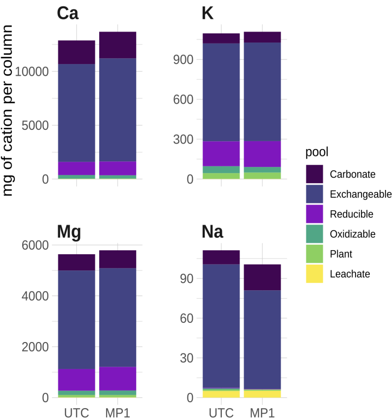
Figure 6: Cation mass-balance. Total mass of cations (in mg) per column, and their distribution between measured pools at the end of the 63-day experimental period. The carbonate, exchangeable, reducible, and oxidizable fractions are based on selective sequential extraction measurements.
